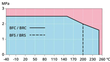
DN 300-800
