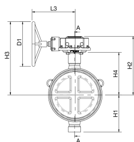
DN 300-800
